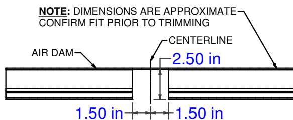
AIR DAM TRIM DIAGRAM
