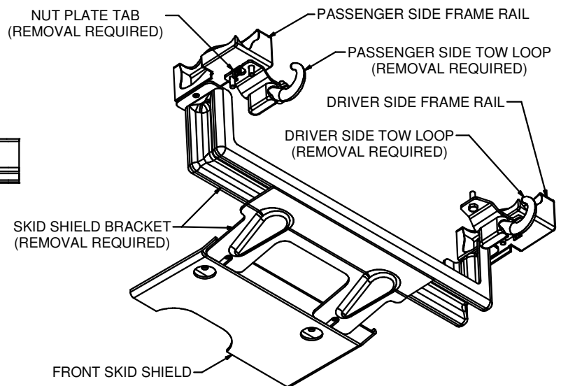
INSTALLATION B PARTS DIAGRAM (BOTTOM VIEW)
