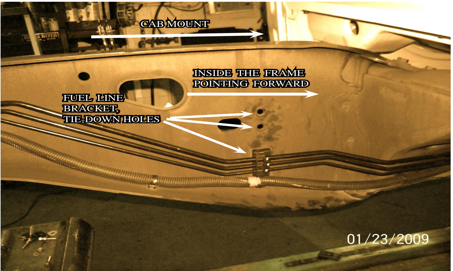
PHOTO C)
