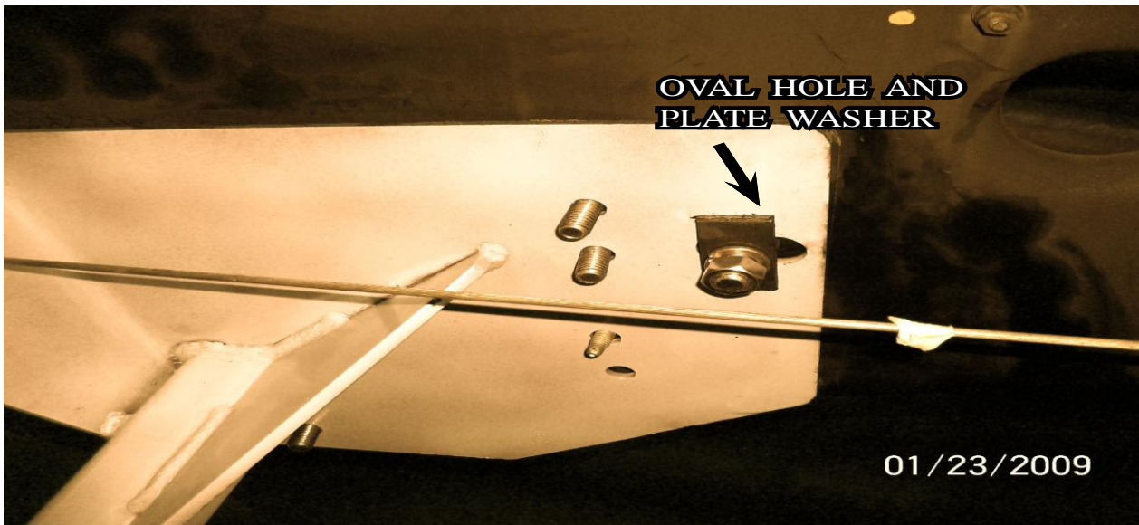
PHOTO L) PASSENGER SIDE
