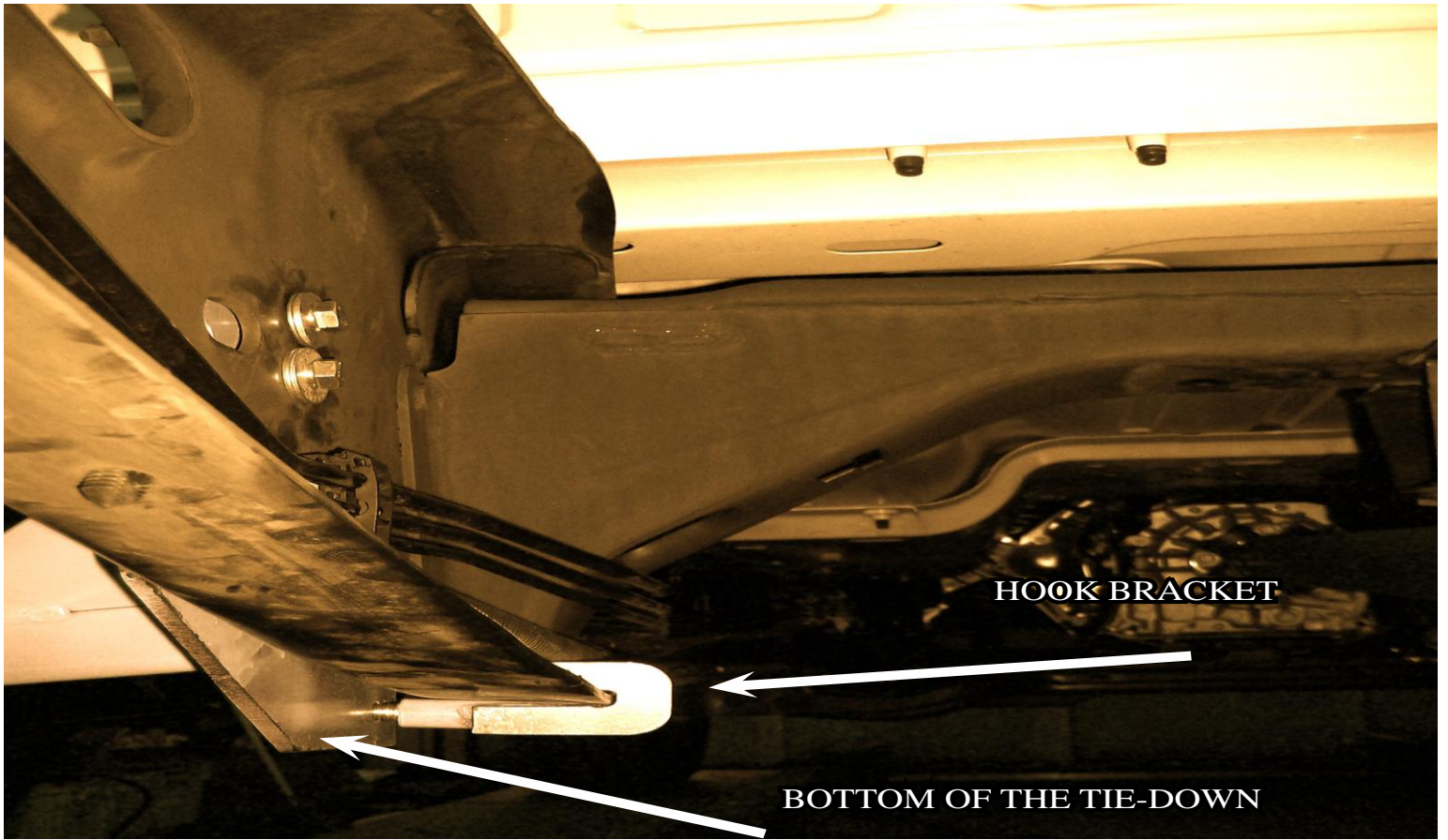
PHOTO I) PASSENGERS SIDE
