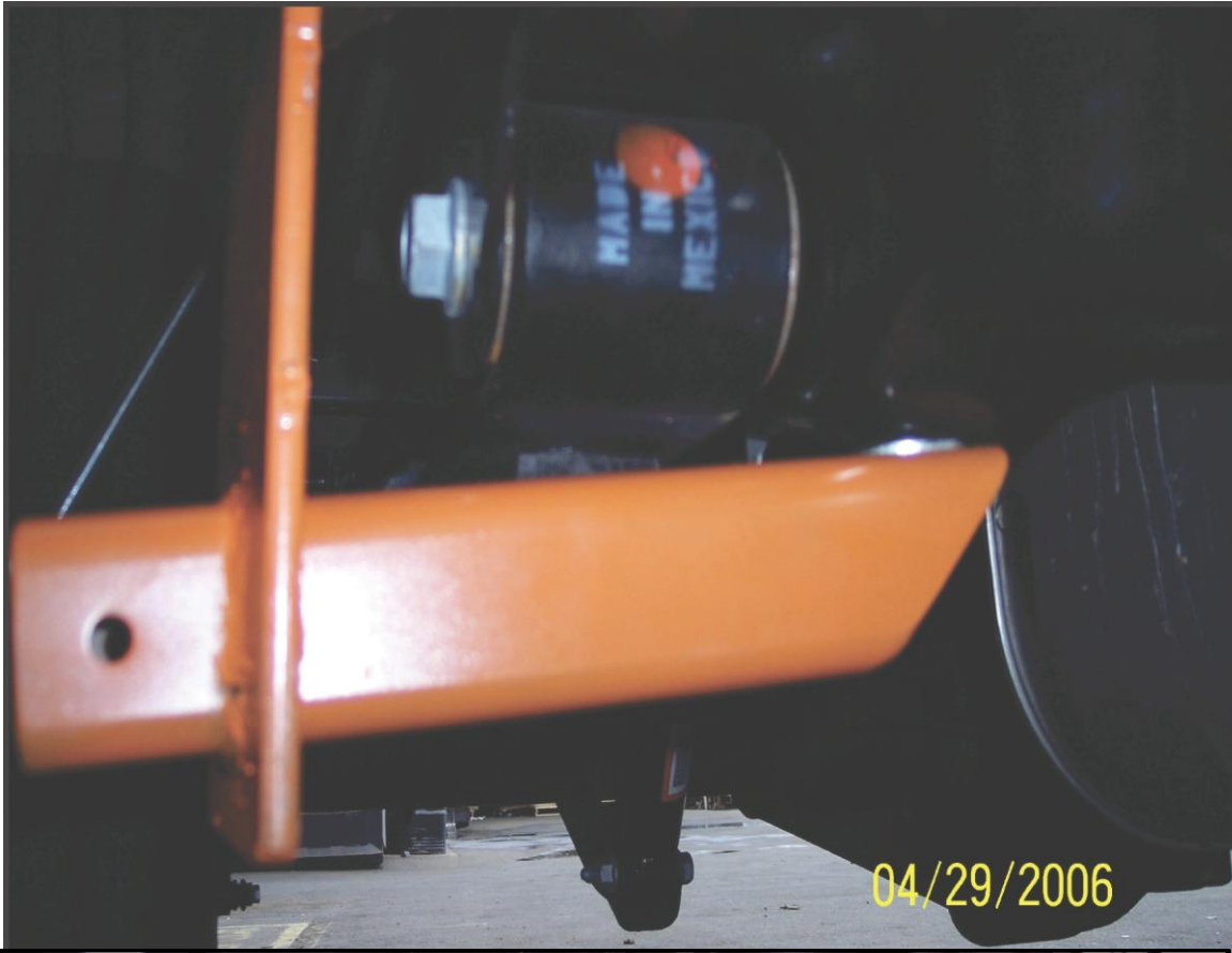
Spring hanger bracket bolt position for step two
