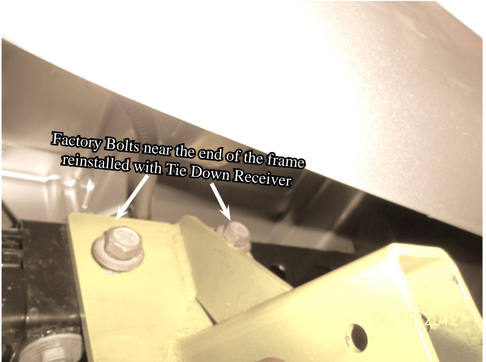
Tie Down Receiver Installed
