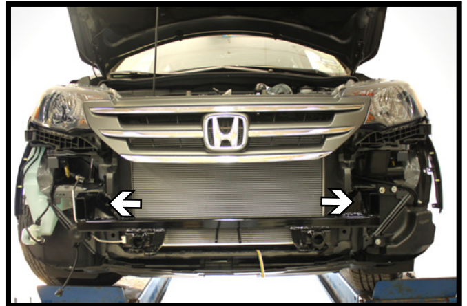
16. Slide the tubes of the baseplate into the rectangular tubing of the vehicle frame.
