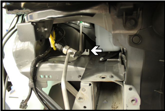
15. On the passenger side, snap the coolant line out of the bracket and carefully move over and out of the way.
